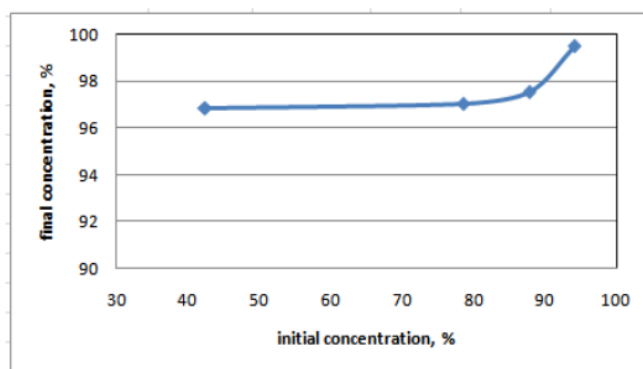
Figure 5. Adsorption at different initial concentration
