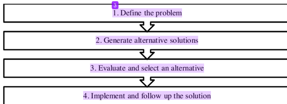
Figure 1. Stages of Formulation of Solutions
