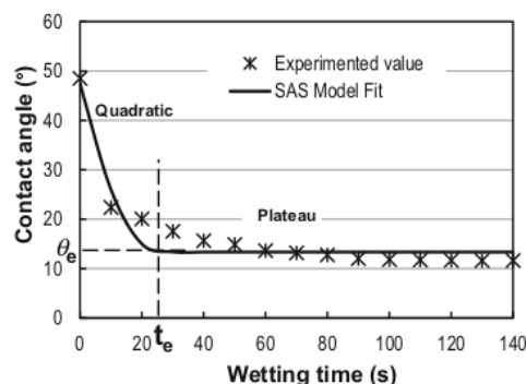
Fig. 1: Determination of the equilibrium contact angle (θ e ) from a plot of the contact angle as a function of time, by segmented regression model
