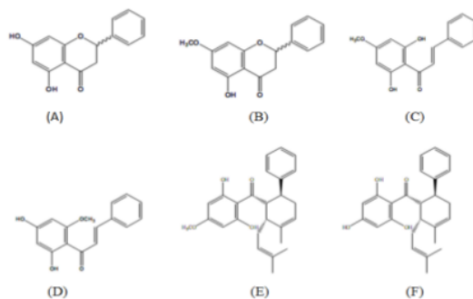
Figure 2. Chemical structure of flavonoid compounds of temu kunci : (A) pinocembrin; (B) pinostrobin; (C) 2', 6' dihydroxy-4'-metoxychalcone; (D) 2', 4'-dihydroxy-6'-metoxychalcone (kardamonin); (E) (-) - panduratin A; and (F) (-) - 4-hydroxy panduratin A
