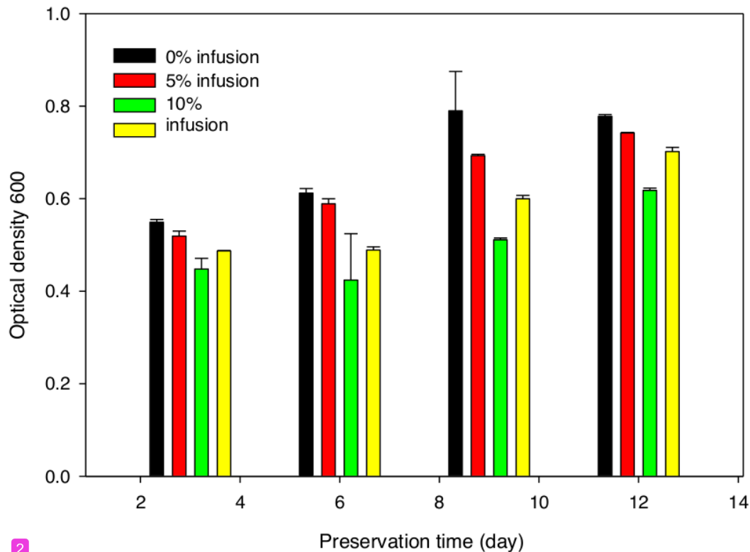
2 Figure 1. The profile of optical density of cultures of meats preserved with infusion of S. polyanthum leaves in NB media
