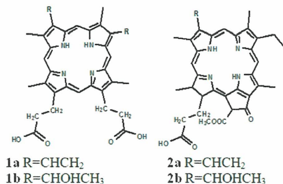
Fig. 1: Molecular structures of protoporphyrin IX (1a), pheophorbide a (2a) and its 1-hydroxyethyl derivatives
