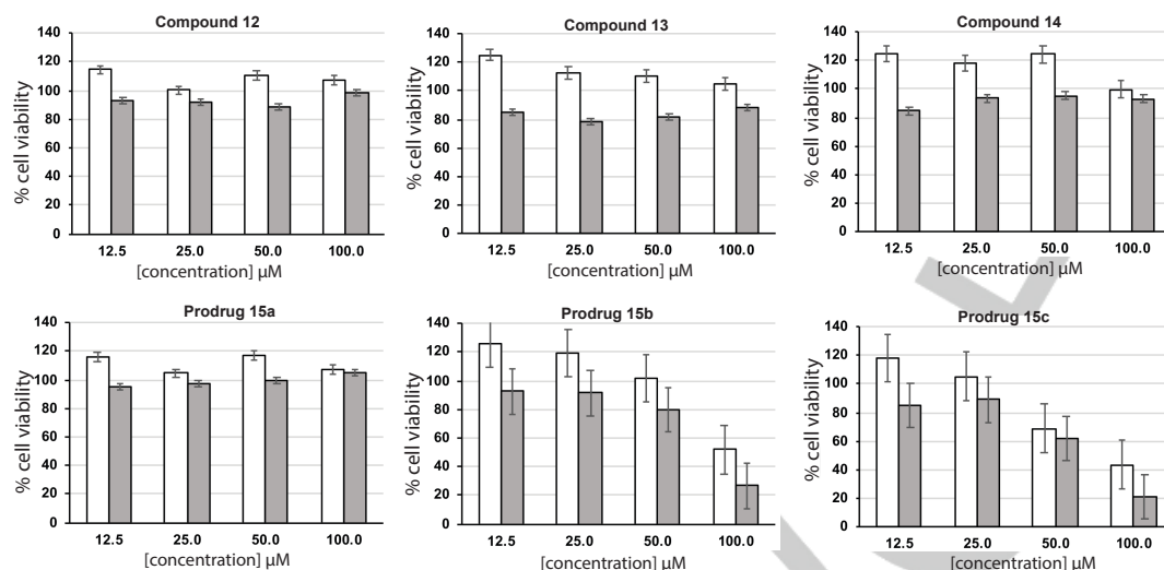
Fig. 3. Cell viability of the unmasked phosphoserine compound ( 12 ), phosphoserine-containing 14-3-3 dimerization inhibitor ( 13 ), its diethyl phosphate derivatives ( 14 ) and the aryloxy triester phosphoramidates ( 15a-c ). Cell viability was determined by standard MTT assay. The compounds were incubated with A549 lung cancer cell line for 48 h (white bar) and 72 h (grey bar) at the indicated concentrations. The percentage of cell viability was calculated and presented as normalized value to control DMSO. Error bars show standard error from triplicate experiments.
