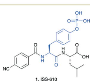
Fig. 2 Chemical structure of the phosphotyrosine containing STAT3 dimerization inhibitor ISS-610.
