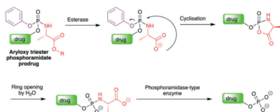
Fig. 1 Metabolism of the aryloxy phosphoramidate prodrug technology to release the monophosphate species.
