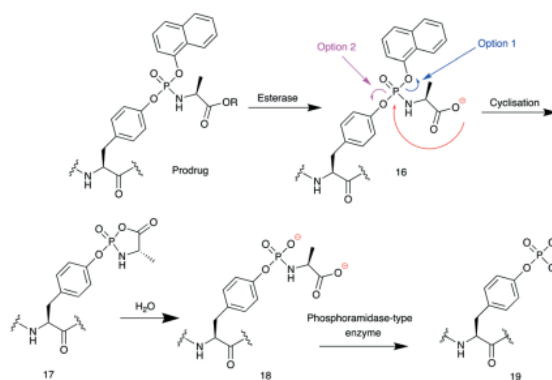
Fig. 5 Postulated mechanism of aryloxy triester phosphoramidate prodrugs. 6
