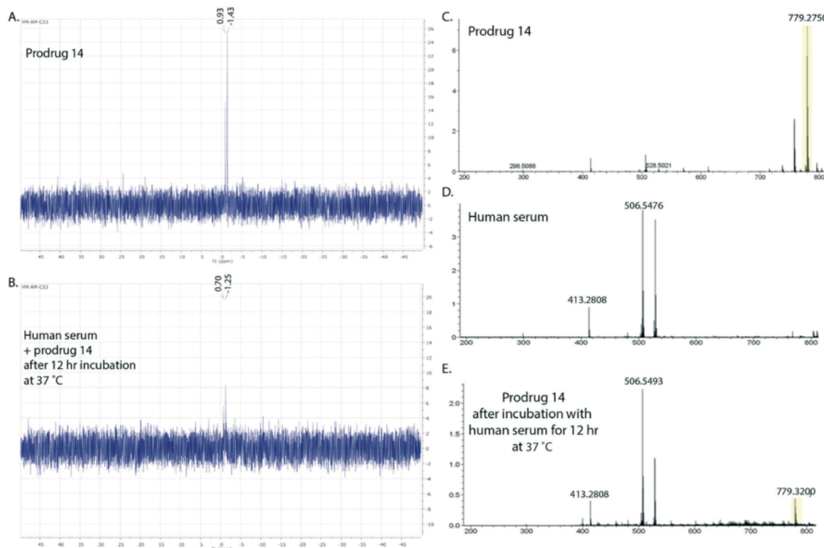
Fig. 6 Human serum stability of prodrug 14 . A: ^{31}\text{P} -NMR scan of prodrug 14 in 0.15 mL DMSO and 0.15 mL \text{D}_2\text{O} . \delta_{\text{p}} = -1.43 and 0.93 . B: Final ^{31}\text{P} -NMR scan of the sample from A after being incubated with 0.3 mL of human serum at 37^\circ\text{C} for 12 h. C: LCMS trace of prodrug 14 alone. The peak corresponding to the mass of the parent compound, 779.2750 \text{ g mol}^{-1} (+Na), is highlighted in light yellow. D: LCMS trace of the human serum alone. E: LCMS trace of the organic fraction of the sample of prodrug 14 after being incubated with 0.3 mL of human serum at 37^\circ\text{C} for 12 h. The peak corresponding to the mass of the parent compound, 779.2750 \text{ g mol}^{-1} (+Na), is highlighted in light yellow.
