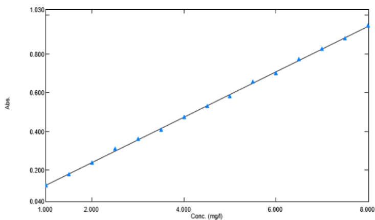
Figure 3. The calibration curve of PGV-0 in methanol.
