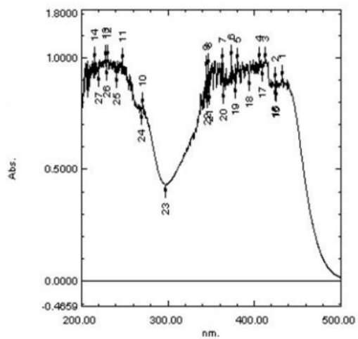
Figure 2. Spectrum of labrasol in methanol.
